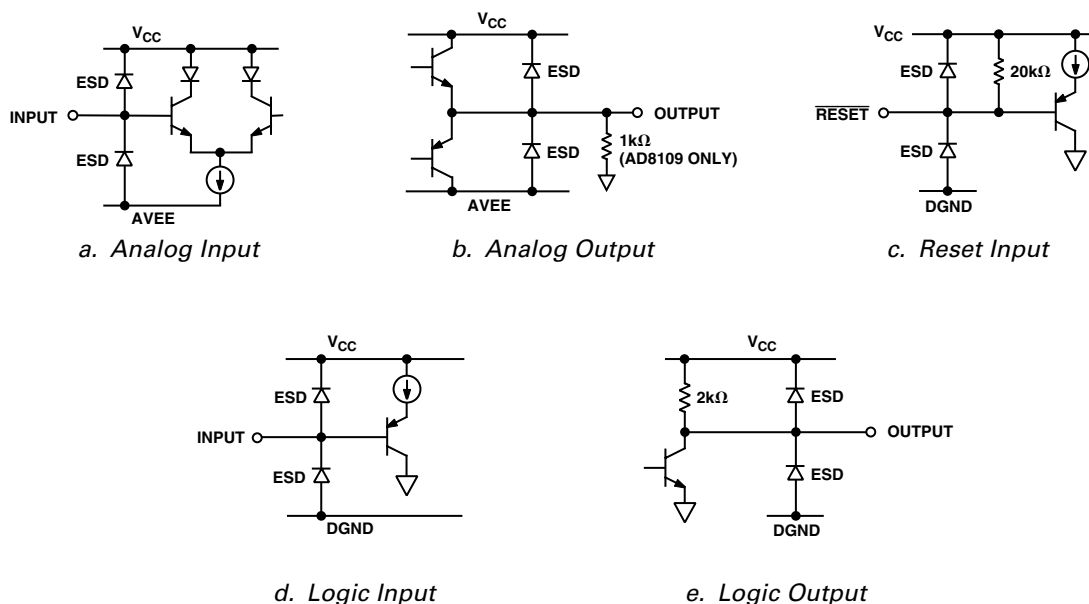
Figure 5. I/O Schematics
